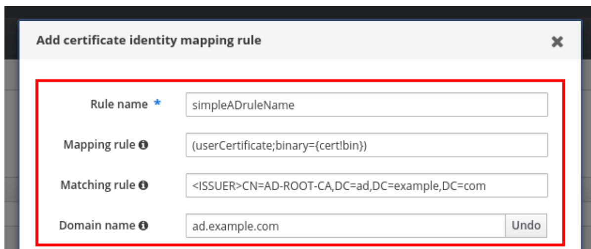
Figure 9.6. Certificate mapping rule for a user with a certificate stored in AD
