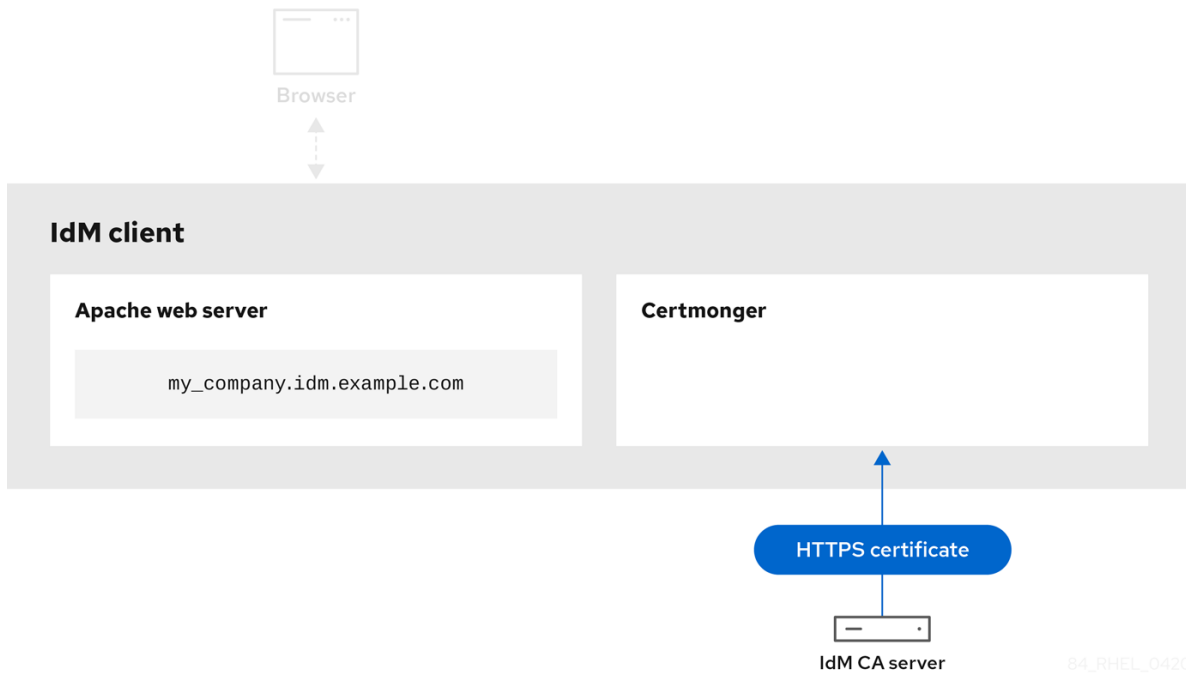
Figure 18.3. IdM CA issuing the service certificate
