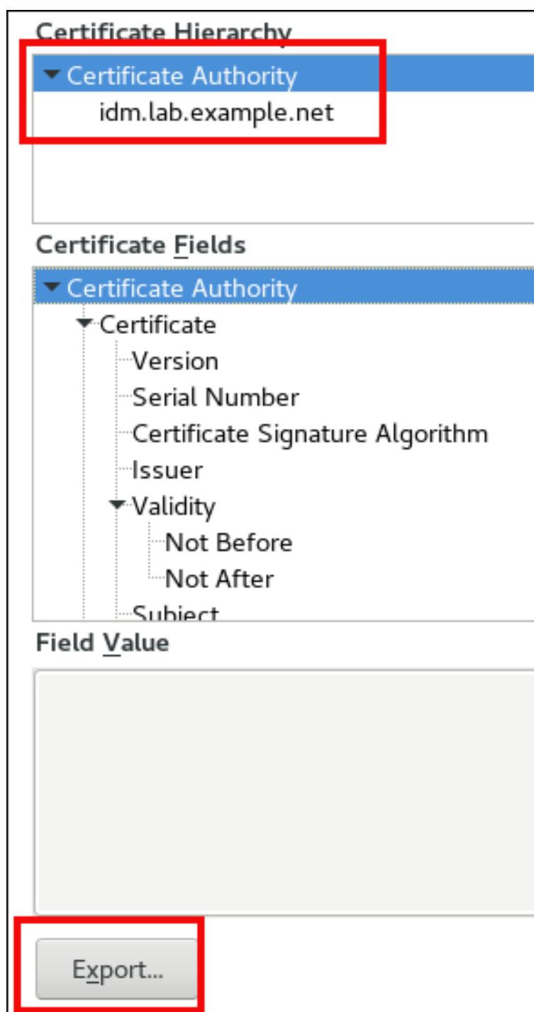
Figure 10.5. Exporting the CA Certificate
