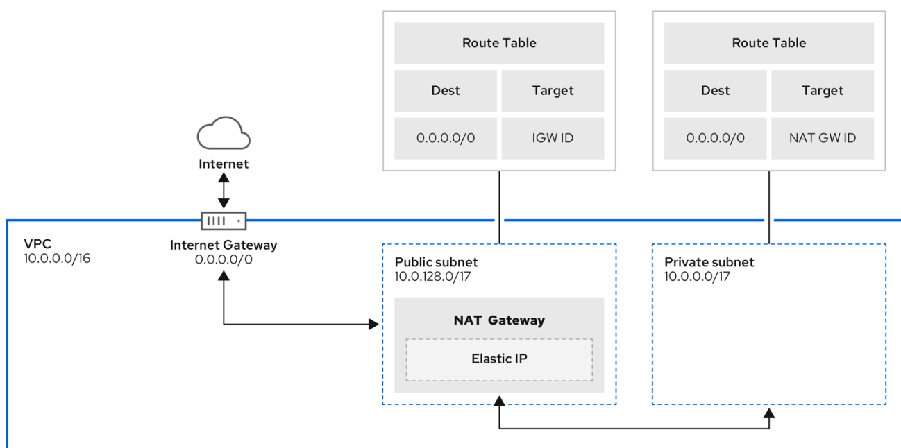
Figure 11.1. Sample VPC Architecture
